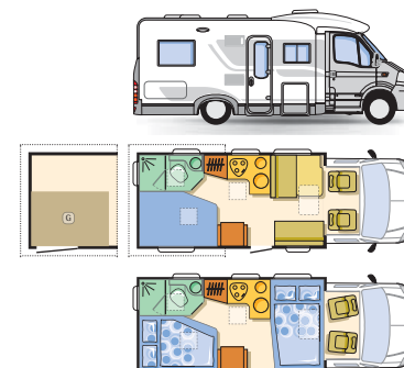
S 687 SP
